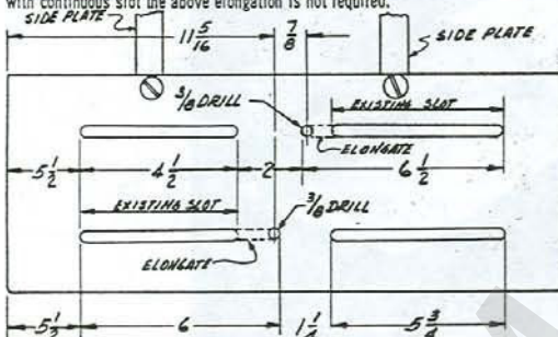
Figure 2 - Entrance Table Detail Model 8900
