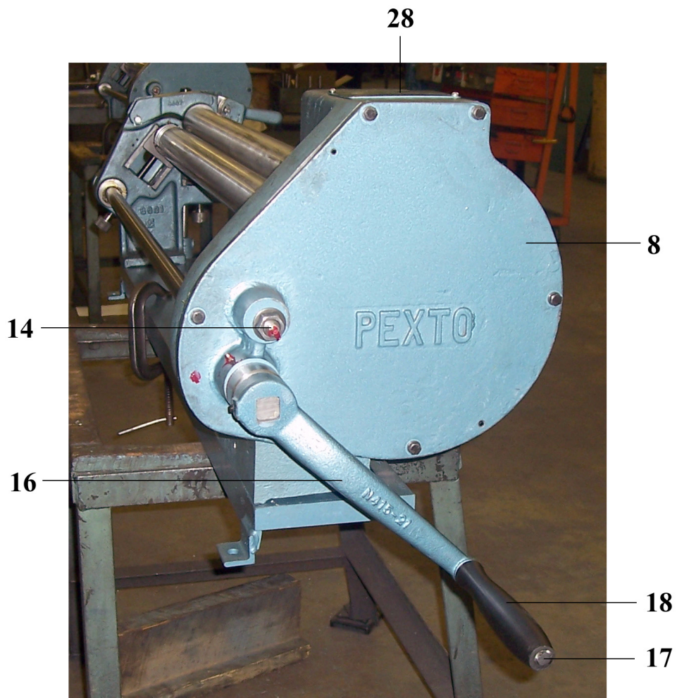
END VIEW (Completely Assembled)
